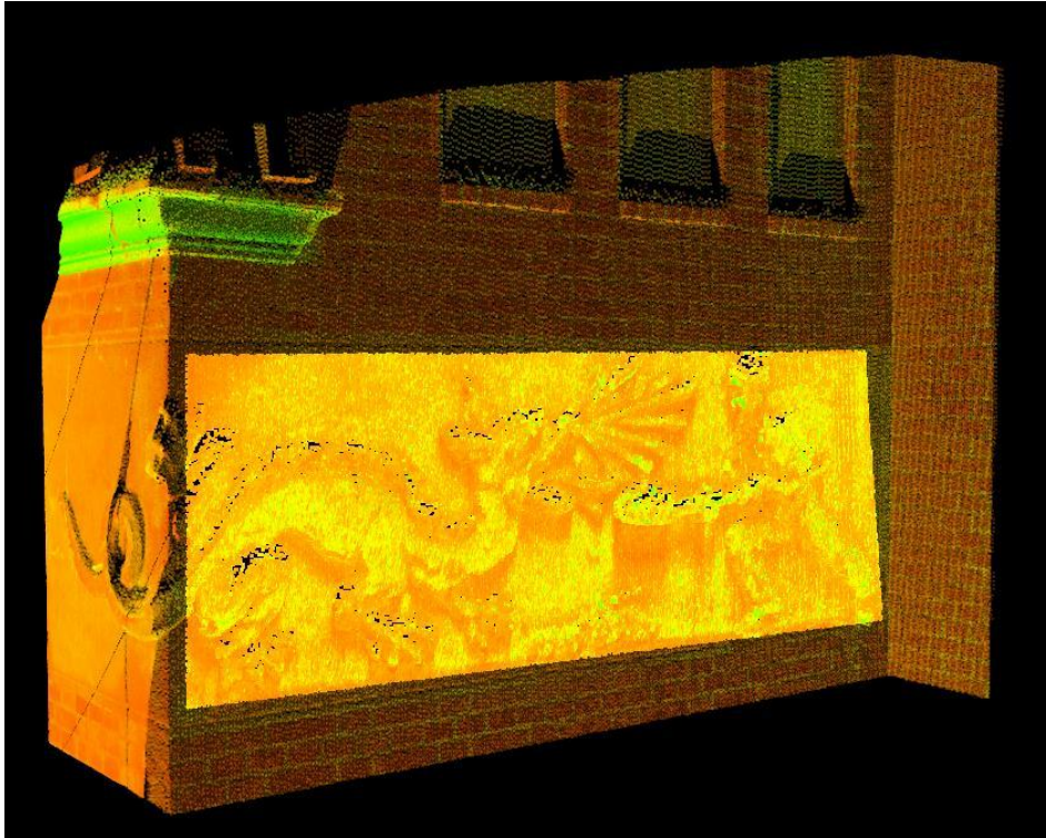
Fig. 4. Option1 - area chosen for unification (source: own research in Cyclone)
