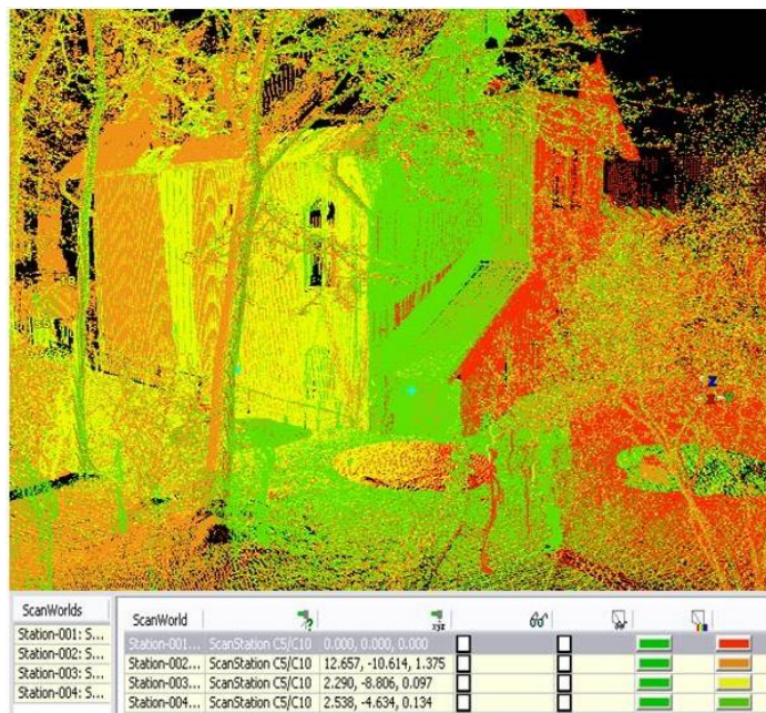
Fig. 3. Obtained point clouds (source: own research in Cyclone)
