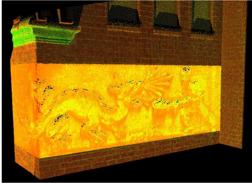
Fig. 6. Option2 - selected object for unification (source: own research in Cyclone)
