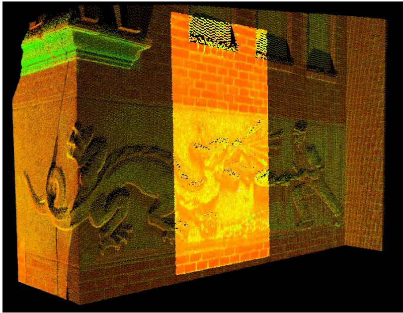
Fig. 8. Option 3 - the selected fragment to unification (source: own research in Cyclone)
